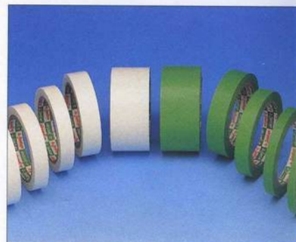
# T501, #6001, #6002 Double Sided Tissue Tape Application: Industrial Use, Name Plate, Electronic Parts, Paper Splicing Standard Width: 12mm, 18mm, 24mm, 36mm, 48mm Standard Length: 10m, 15y, 50m Adhesive: Acrylic Solvent
