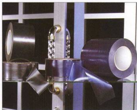
# 801 PVC Surface Protective Tape Standard Width: 18mm - 1250m Standard Length: 90m Thickness: 0.13mm Colour: Transparent Blue, White, Black Adhesive: Solvent Rubber
